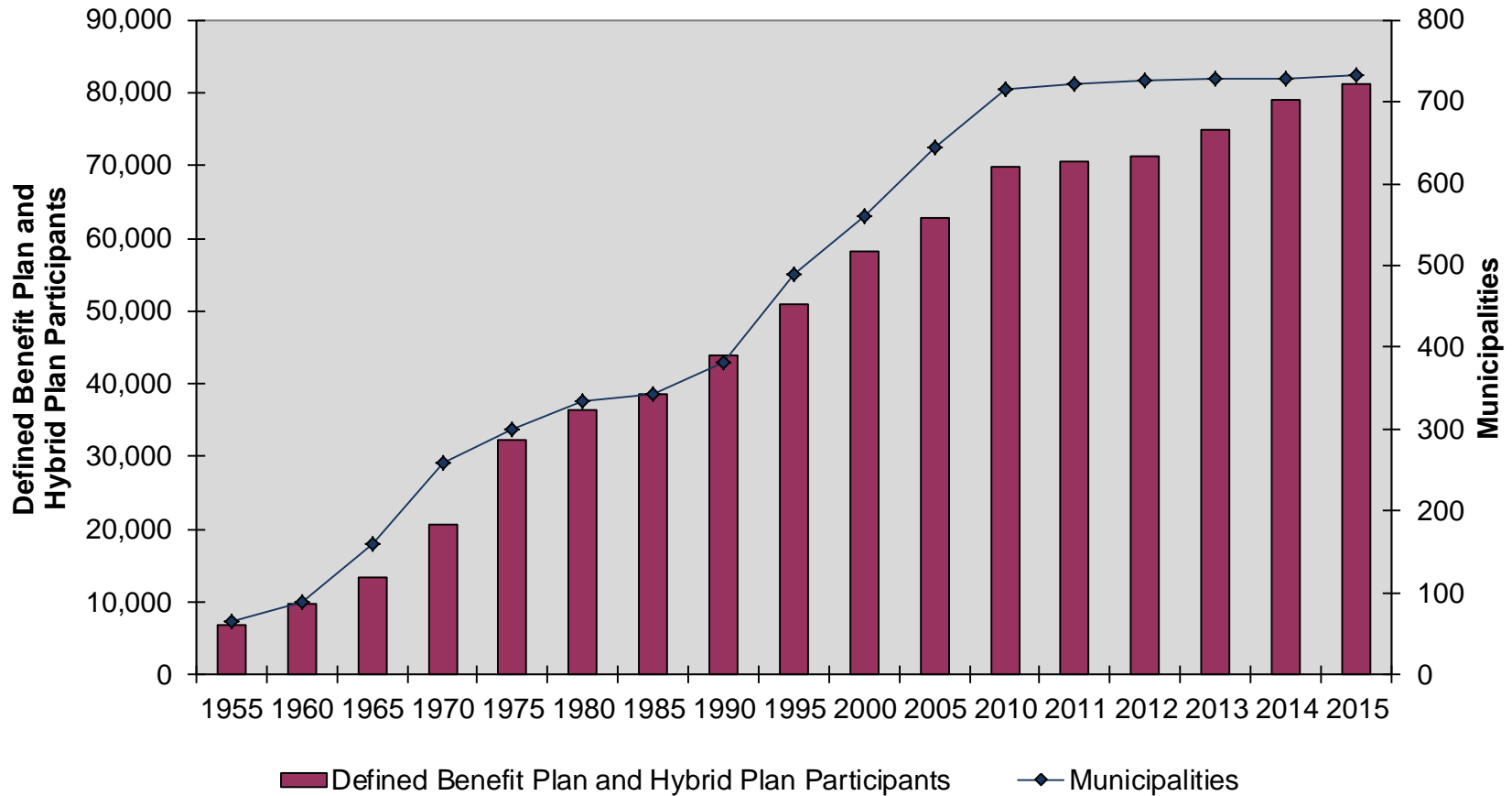
Chart 1 MERS Growth
